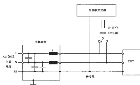
图2 依据 IEC 61000-4-5: 2005 Figure 6
