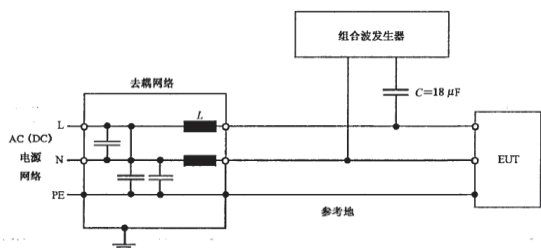
图1 依据 IEC 61000-4-5: 2017 Figure 5
