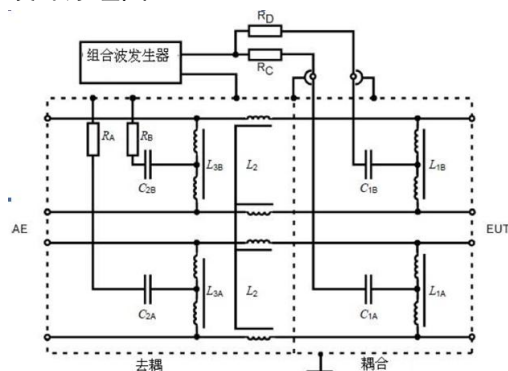
依据 IEC 61000-4-5: 2017 Figure 11
