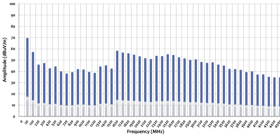
COMB GENERATOR OUTPUT (amplitude vs frequency)
