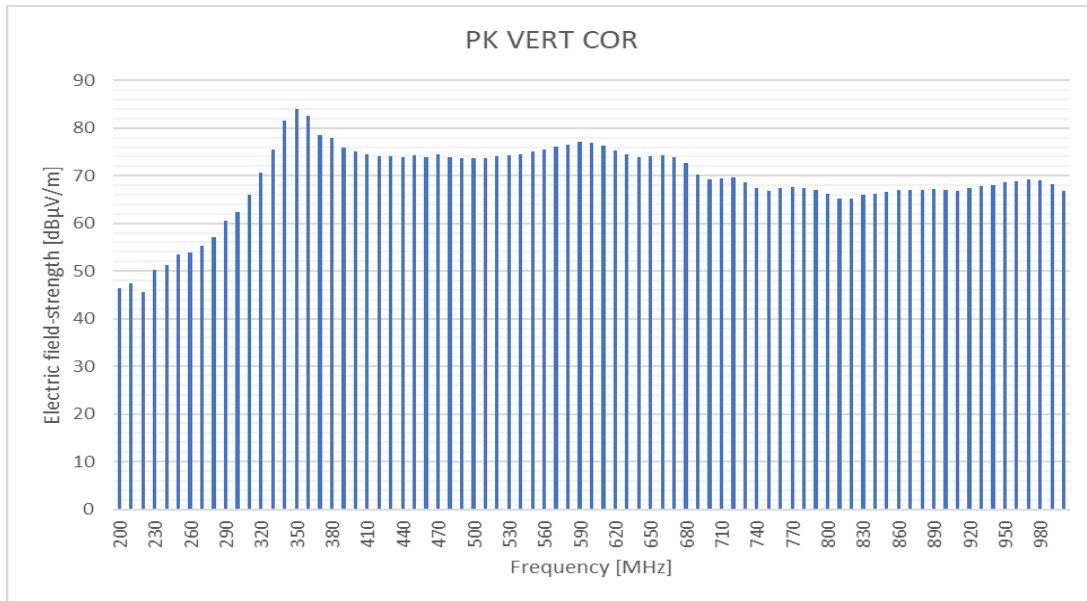
Measured with logarithmic periodic antenna, 3m distance, 1 meter height
