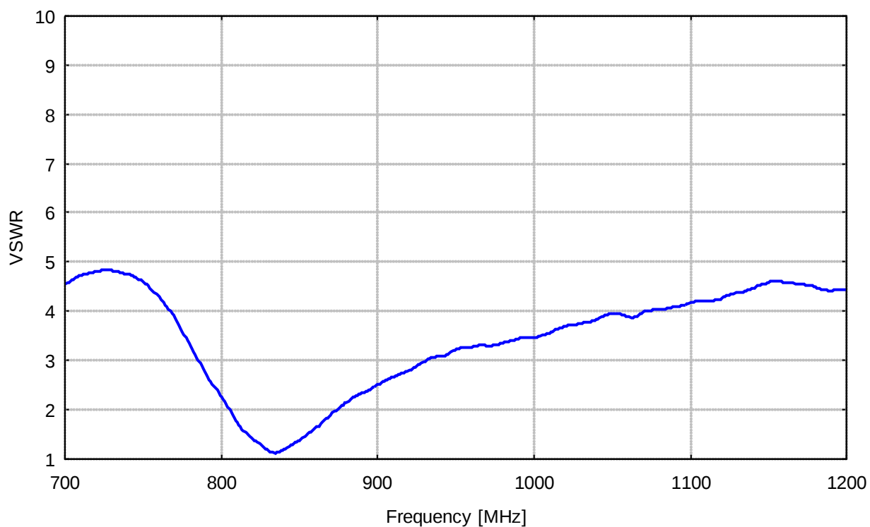
TSA 835 typical VSWR
