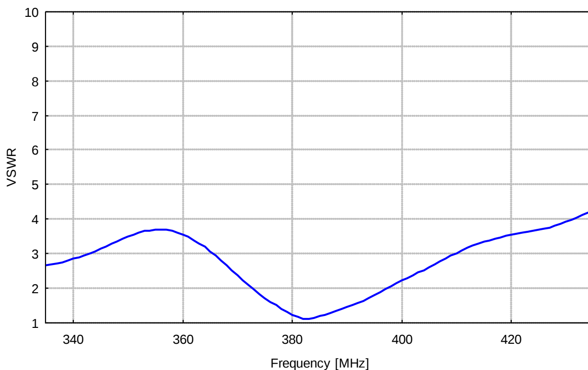
TSA 430 typical VSWR
