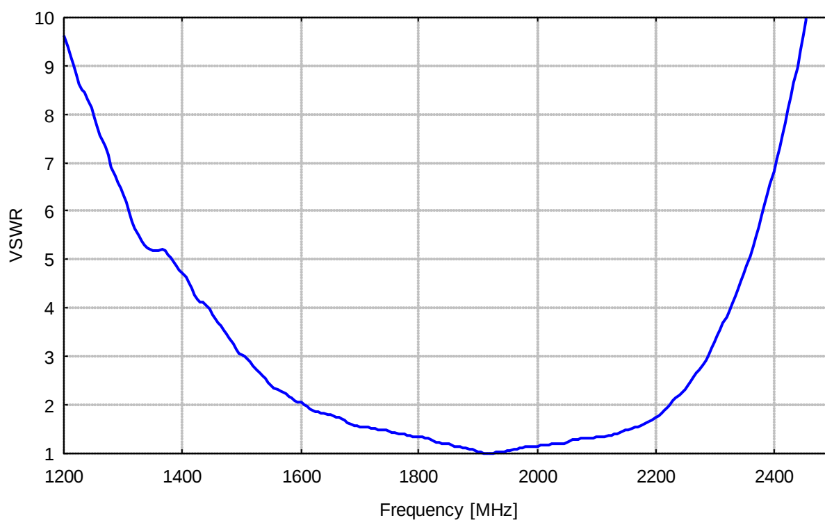
TSA 1950 typical VSWR
