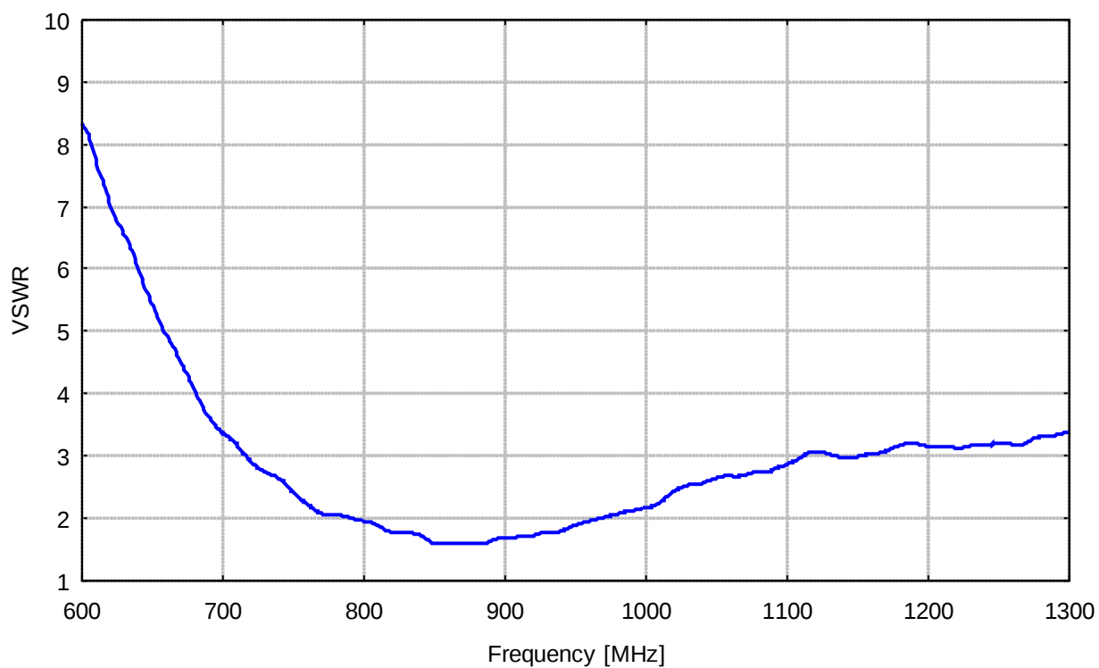
TSA 880 typical VSWR
